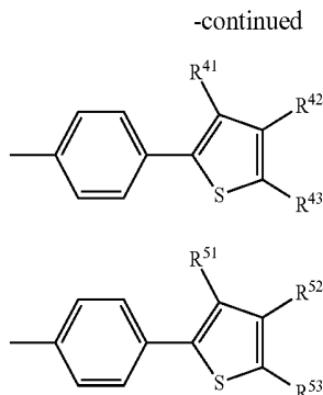
General Formula (4)
