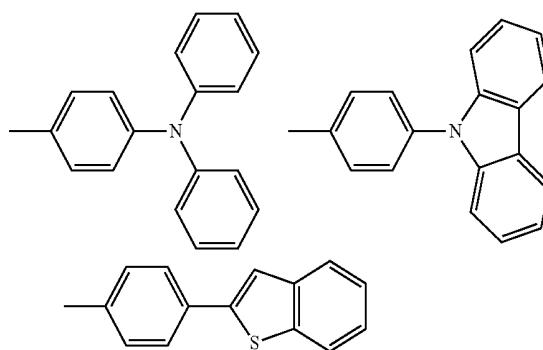
General Formula (2)
