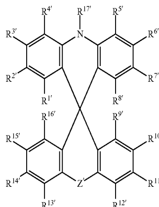
[Chem. 7]
