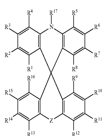
General Formula (1)
