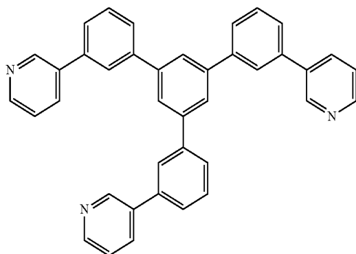
TmPyPB
